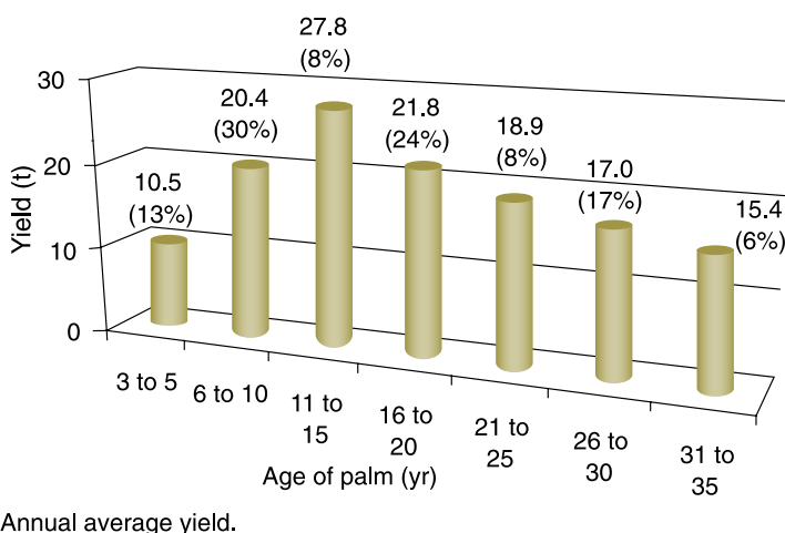
Figure 1. Yield of fresh fruit bunch (FFB) based on age profile (2006/2007).
