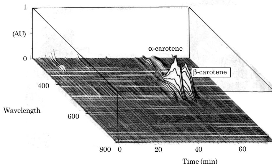
Figure 2. A 3D chromatogram of palm carotenoids.
