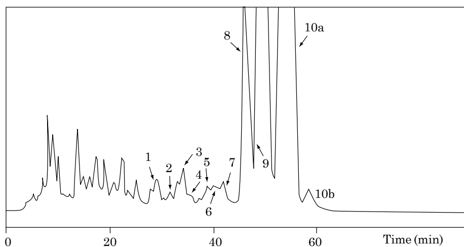
Figure 1. Crude palm oil carotenoids scanned at 444 nm. The peak numbers here are the same as those in Table 1. Note: phytoene and phytofluene are not shown in this chromatogram because they are detected only at 286 and 347 nm respectively.
