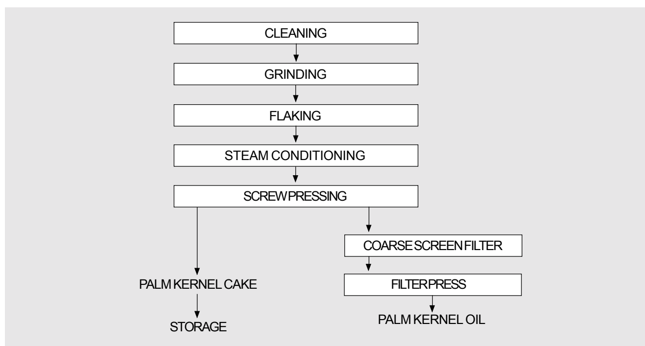
Figure 1. Mechanical extraction of palm kernel oil.
