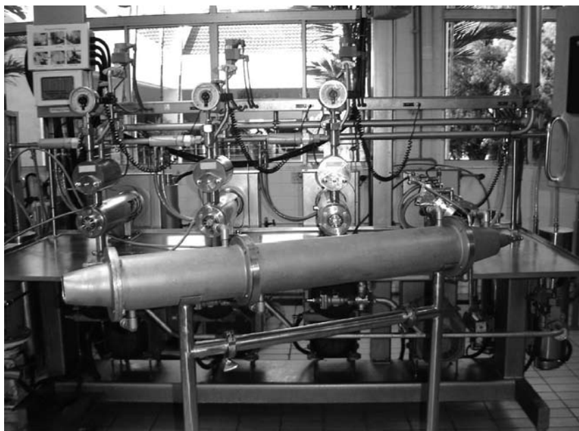
Figure 2. Pilot plant set-up for the trial runs on palm-based roll-in margarine.
