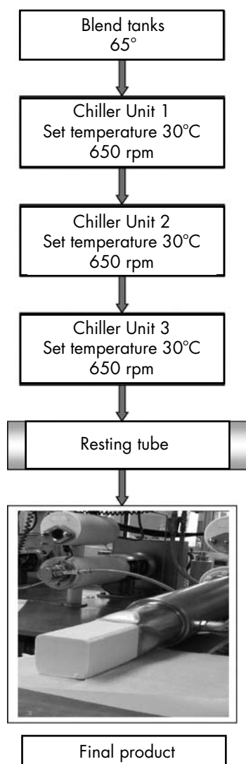
Figure 3. Flow chart of the processing conditions for the production of palm-based roll-in margarine.
