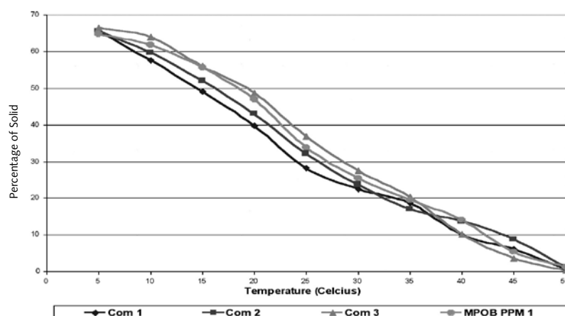
Figure 5. Solid fat contents of commercial and MPOB PPM 1 roll-in margarines.
